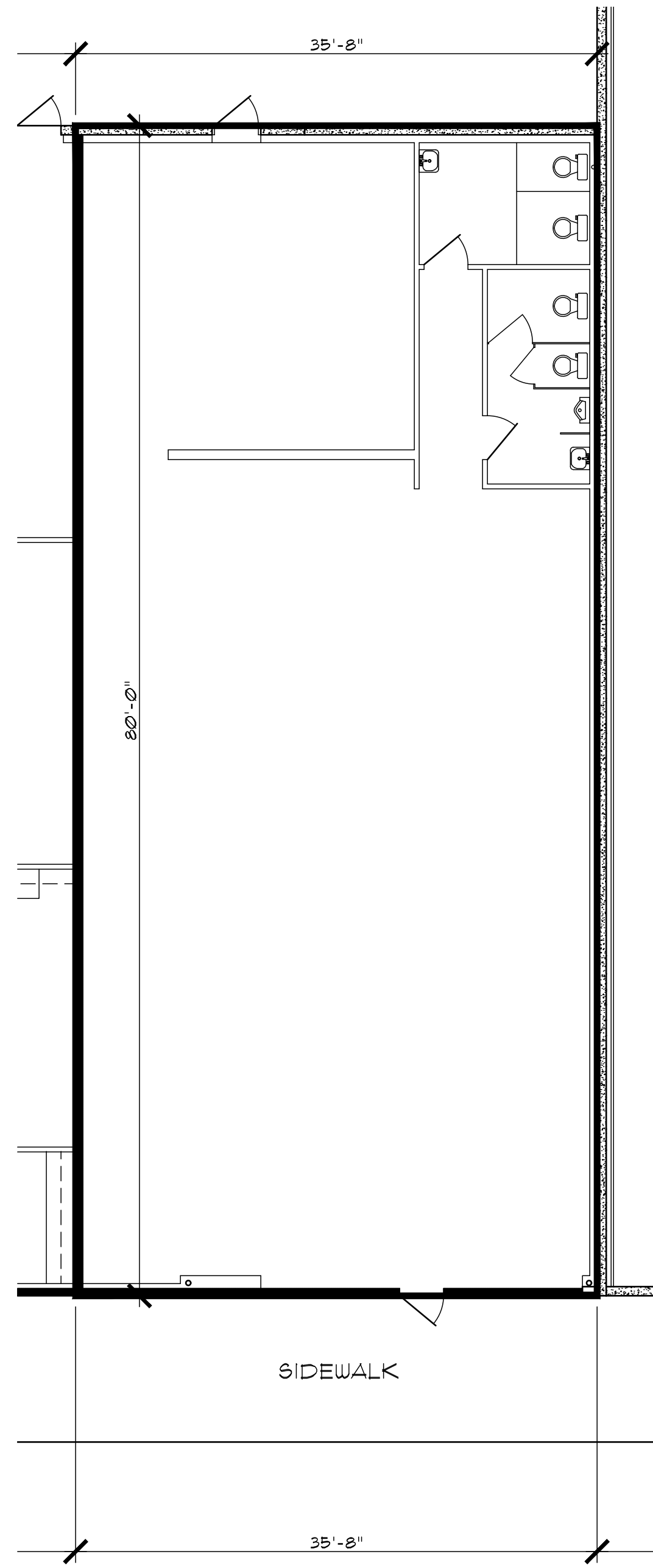
FIRST FLOOR LEASING PLAN - 1810 SCALE: 1/8" = 1'-0"
